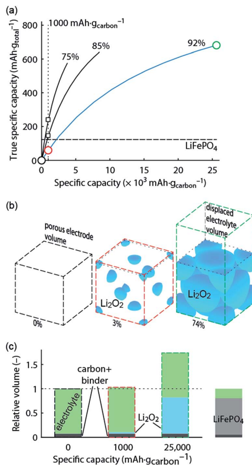
Fig. 1 True electrode capacity with limited capacity cycling. (a) True capacity of a Li- \text{O}_2 cathode as a function cycling capacity per mass of carbon substrate for three cases of initial porosity (percentages above the curves). 4% volume are accounted for the binder, and the carbon volume fraction is adapted to yield the initial porosity. At an initial porosity of 92% a \text{Li}_2\text{O}_2 volume occupation of 74% (fcc packing) corresponds to 80% filling of the available pore space. The same 80% filling of the available pore space is assumed for the other initial porosities. The analogous value for the intercalation material \text{LiFePO}_4 is shown for comparison. (b) Space filling of spherical \text{Li}_2\text{O}_2 inside the porous electrode volume with fixed sphere centres and the displaced electrolyte volume (together with the super-host structure) at 0, 1000, and 25 000 \text{mA h g}_{\text{carbon}}^{-1} , respectively (indicated by the circles in a). Sphere sizes are to scale and the numbers indicate their volume occupation in the porous electrode volume. (c) Volumes of the electrode components at these capacities normalized to the full electrode volume in the delithiated state. Values for a \text{LiFePO}_4 cathode are shown for comparison and demonstrate a very different electrolyte/active material ratio. The figure is adapted from ref. 4 with permission of NPG.
